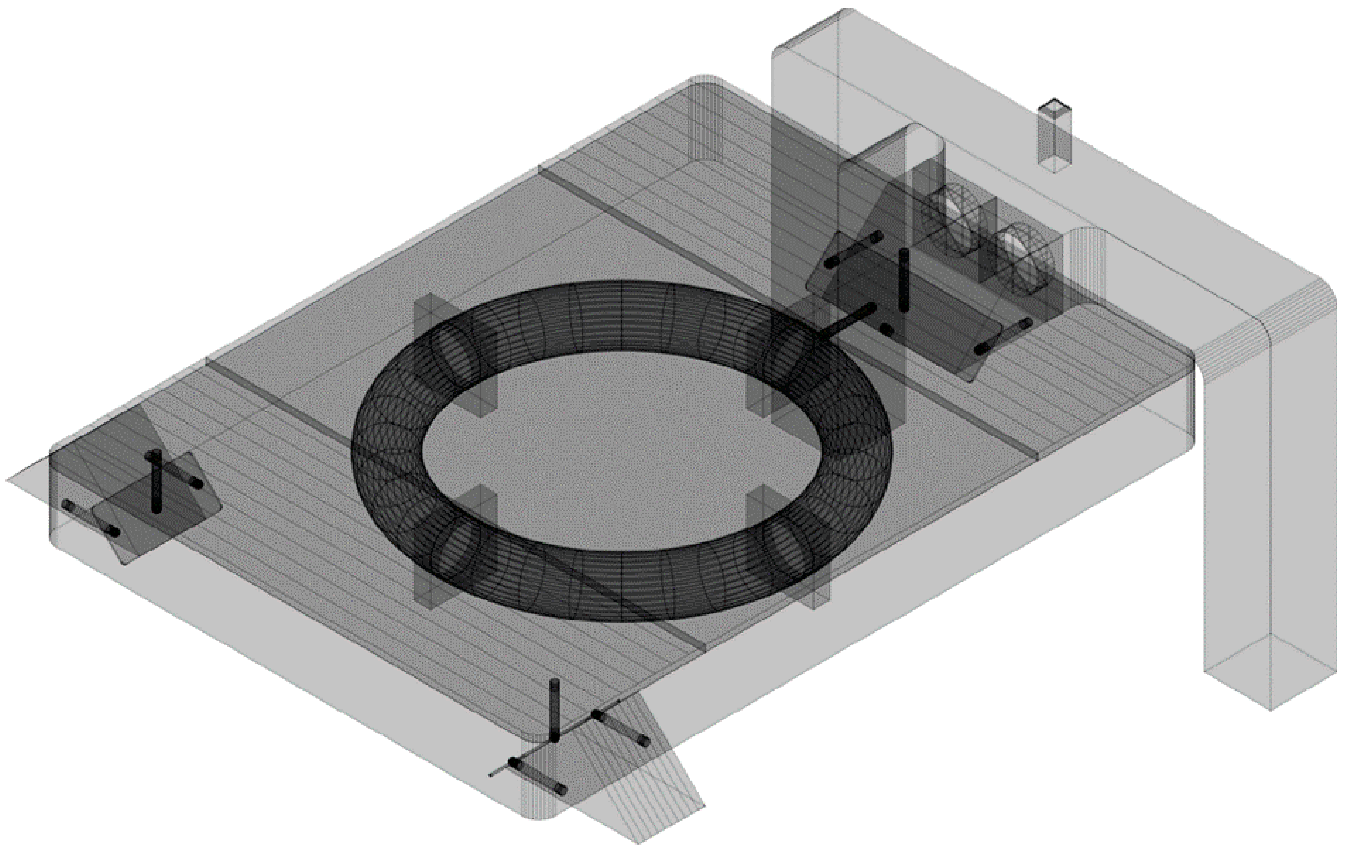
Figure 2. Structure of a solar heating system to maintain the batteries charged. Overview.
